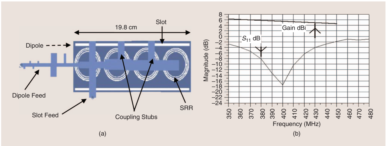
Figure 6. (a) The printed antenna with an SRR and (b) the computed S_{11} and antenna gain.
