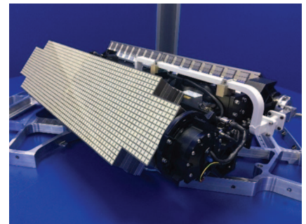
Figure 3. The dual-panel Ku-/Ka-band Gilat SatCom antenna.
