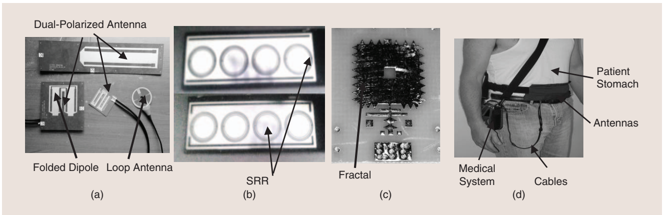
Figure 8. (a) Wearable antennas for medical applications, (b) metamaterial-based antennas, (c) a fractal wearable antenna resonator at 8 GHz, and (d) wearable antennas mounted on patient.
