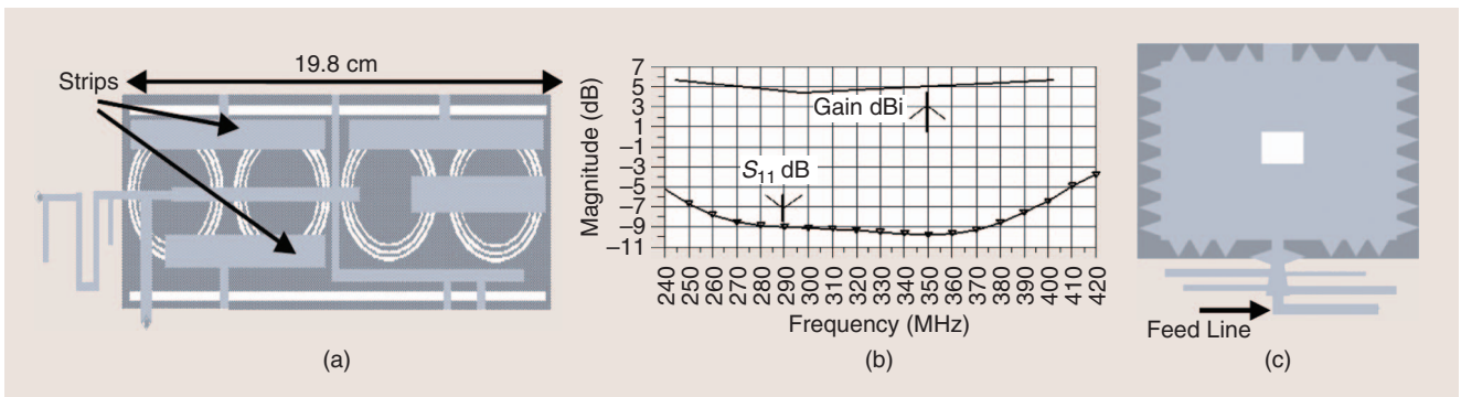
Figure 7. (a) The antenna with metallic strips, (b) the S_{11} and antenna gain, and (c) the fractal patch. Figure 8 presents photos of the antenna in wearable forms.
