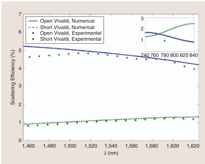
Figure 5. The antenna scattering efficiencies as a function of wavelength.
