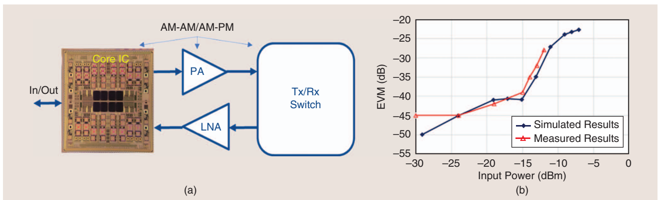
Figure 10. (a) A simplified block diagram of the core IC and (b) the EVM results.
