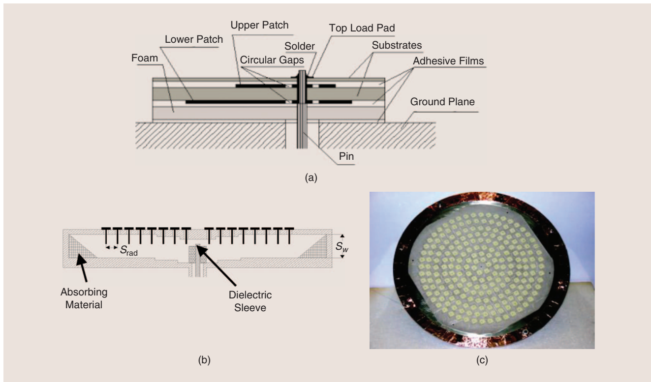
Figure 1. The geometry of the dual-frequency, dual-circular-polarization microstrip antenna: (a) the element, (b) the array cross section, and (c) a photo of the antenna.
