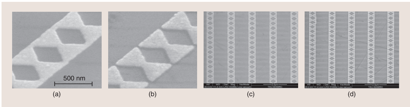
Figure 4. SEM images of the fabricated (a) short-circuit array and (b) open-circuit array. (c) and (d) show zoom outs of the arrays.
