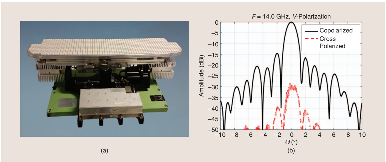
Figure 2. (a) The SPA PAC system and (b) the SPA radiation pattern at 14 GHz.
